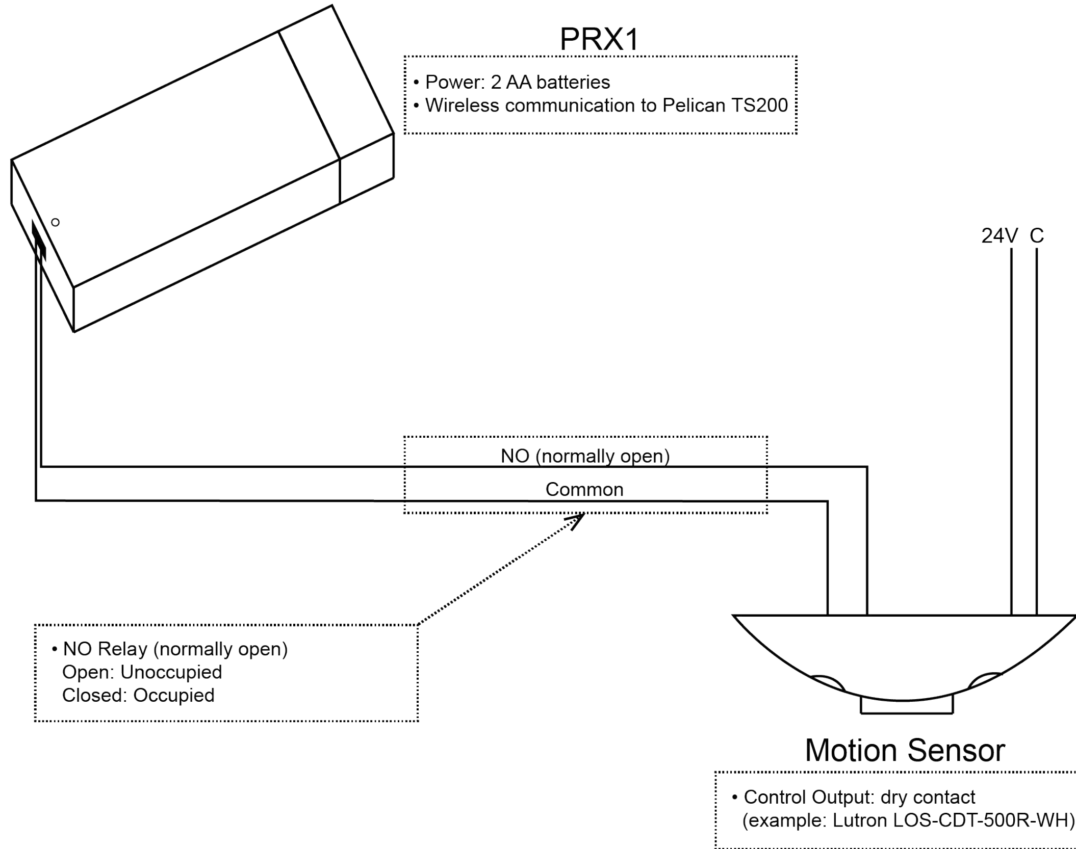
PRX1 Wireless Proximity Sensor + Motion Sensor Wiring Diagram
