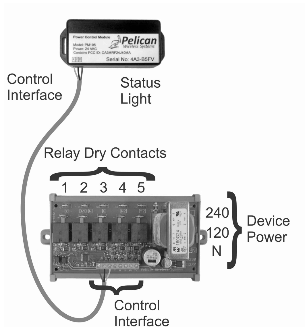
Wiring configuration
